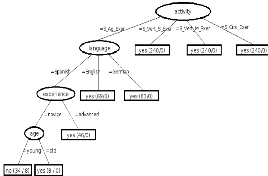
Fig. 1. Decision tree in the example 1
