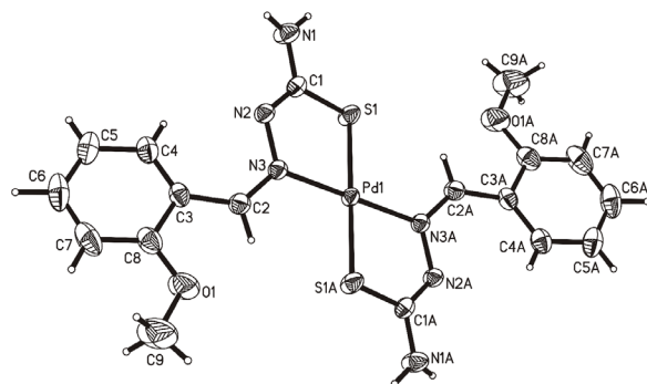
Fig. 1. Molecular structure of Pd(TSC 3 ) 2 ( 7 ) in the crystal. The displacement ellipsoids are drawn at the 50% probability level, hydrogen atoms with arbitrary radii.
