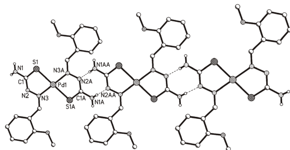
Fig. 2. One-dimensional chain structure of Pd(TSC 3 ) 2 ( 7 ) in the crystal.
