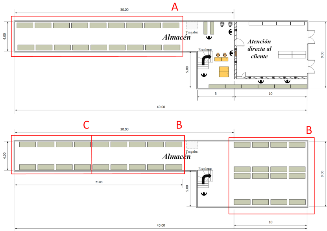
Figure 8. Optimized plan of the two warehouses according to ABC groups
