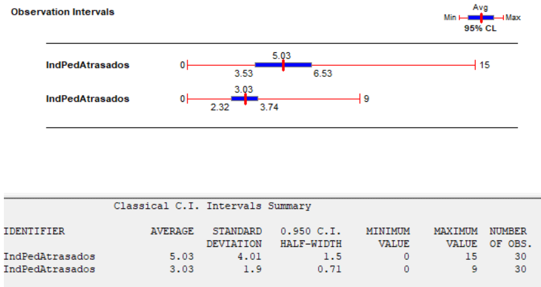
Figure 12. Comparison between current scenario and 20% reduction of picking time
